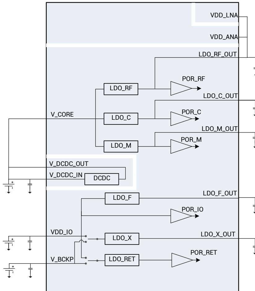
图 5-1 DC/DC bypass 时供电和时序 (Main Supply 是 1.2V~1.98V)
